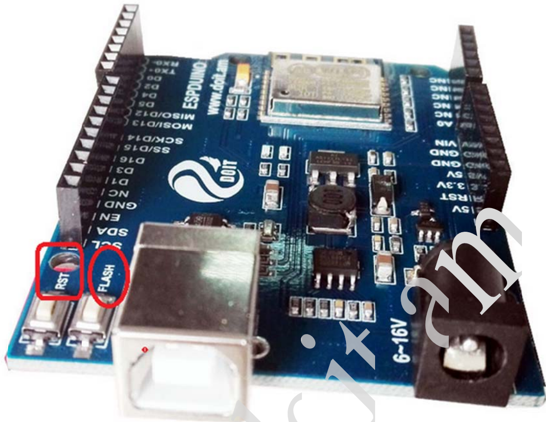
Figure Buttons on ESPduino
