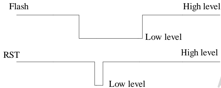
Figure Principle of Press Button
